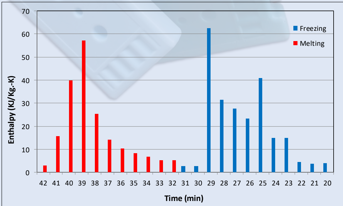
Figure 1: Enthalpy of IP39 against temperature
