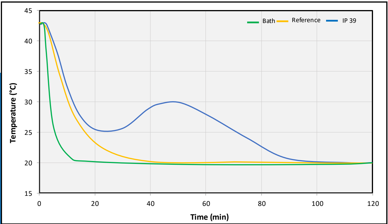
Figure 2: Freezing Curve of IP39
